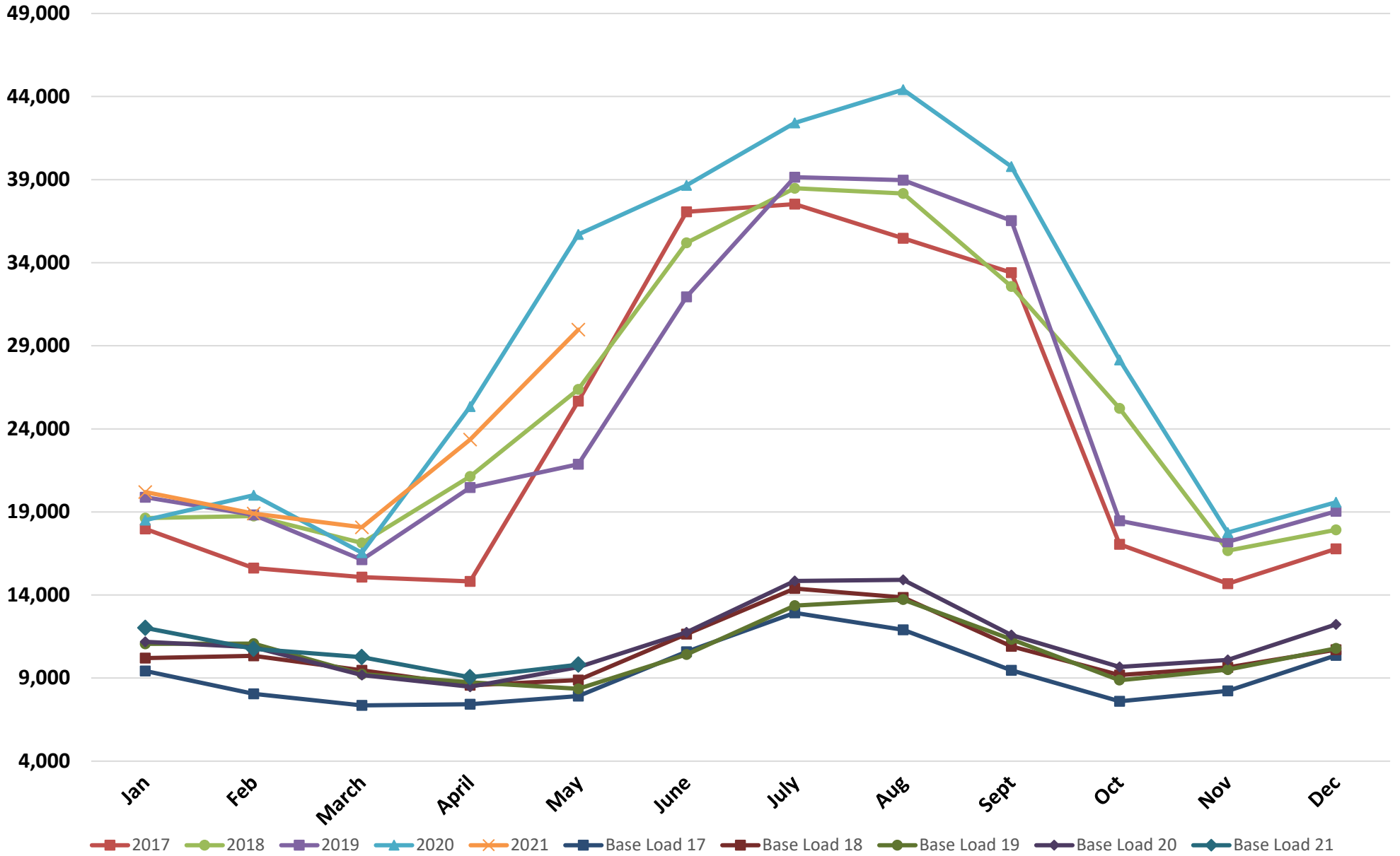
2017 - 2021 KW LOAD
